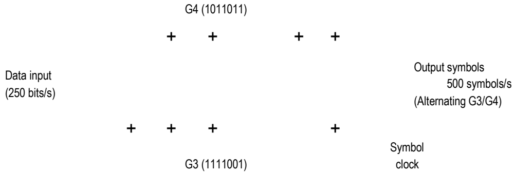
Figure B-11. Convolutional encoding
