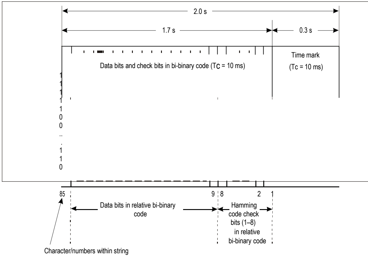
Figure B-10. Data string structure
