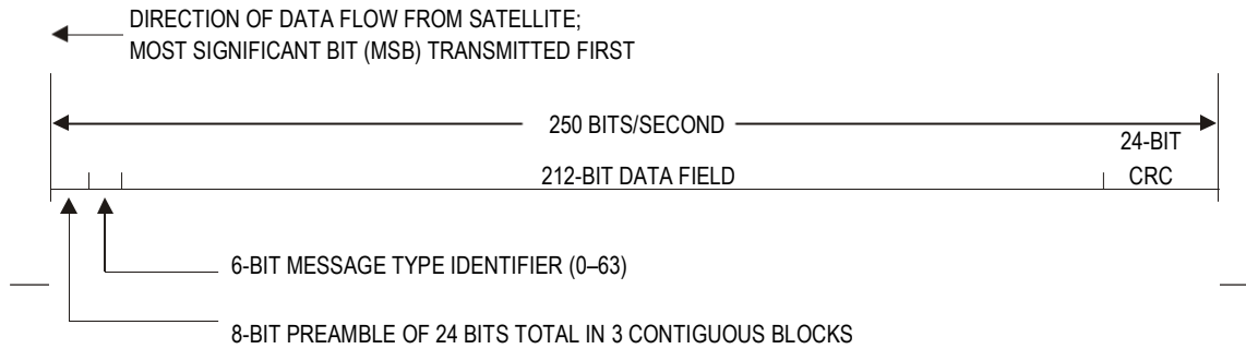
Figure B-12. Data block format
