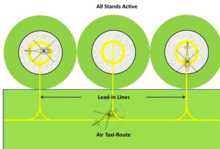
Figure 3-5. Turning stands with air taxi-routes/simultaneous use
