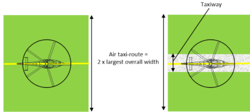
Figure 3-3. Helicopter air taxi-route and combined air taxi-route/taxiway
