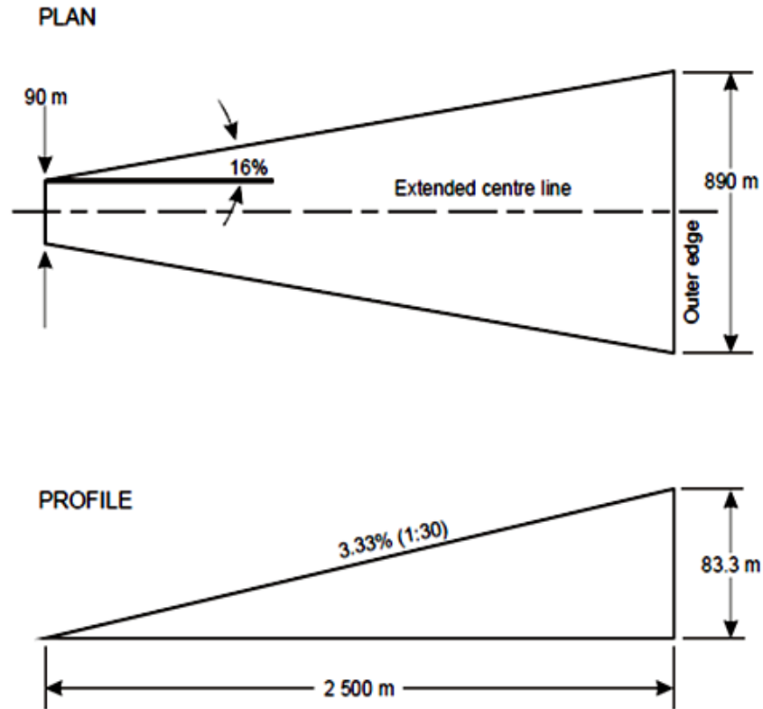
Figure A2-4. Approach surface for non-precision approach FATO
