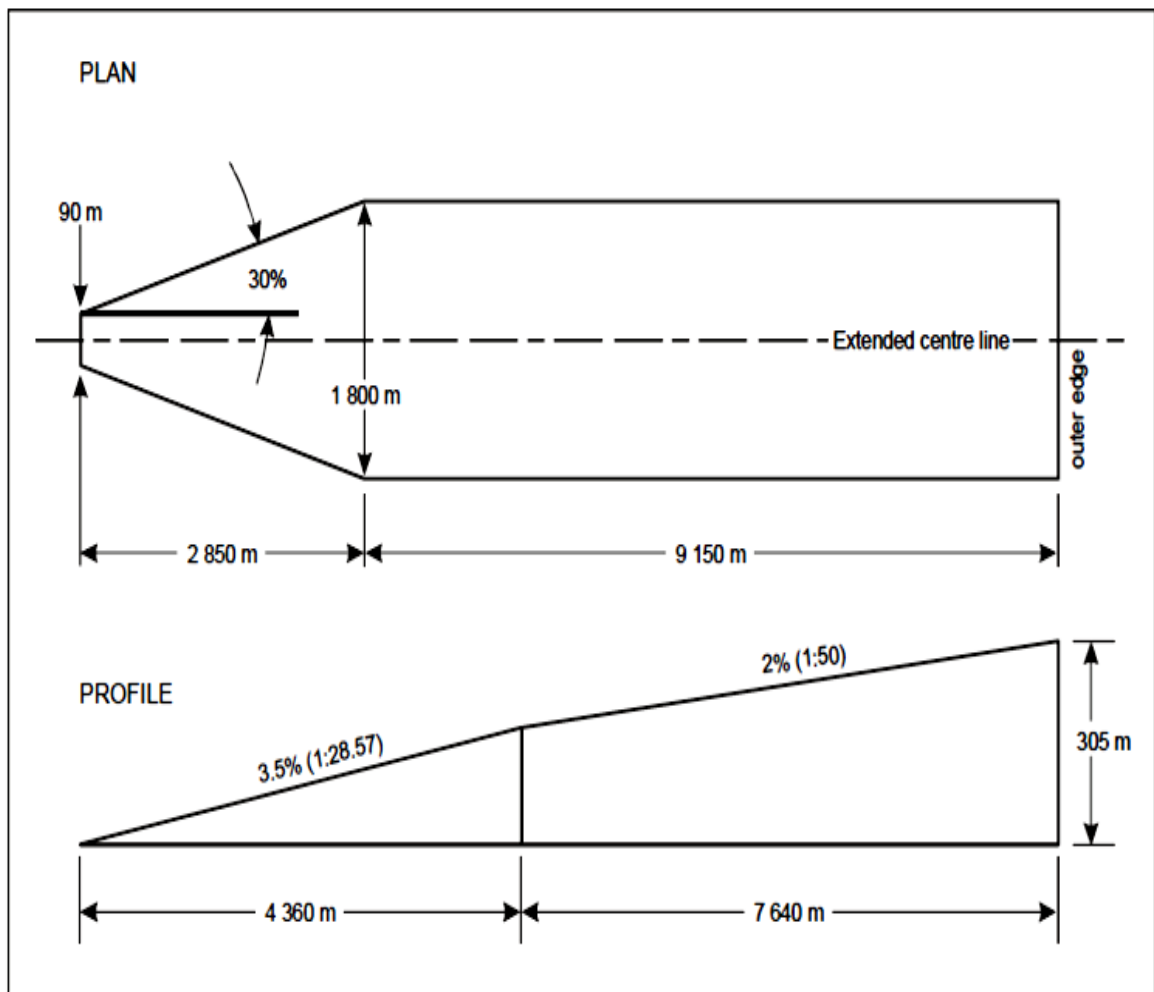
Figure A2-2. Take-off climb surface for instrument FATO
