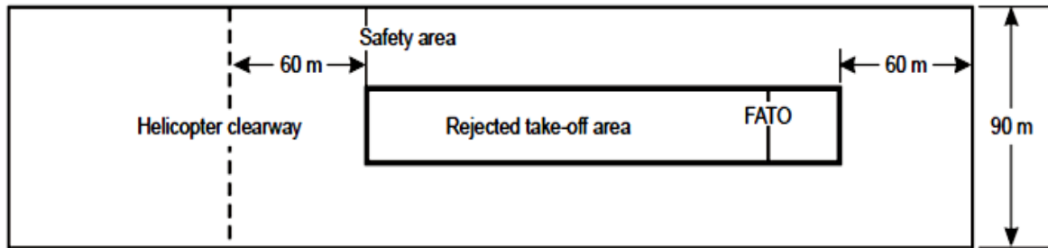
Figure A2-1. Safety area for instrument FATO
