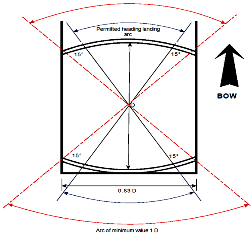
Figure 3-7. Shipboard permitted landing headings for limited heading operations
