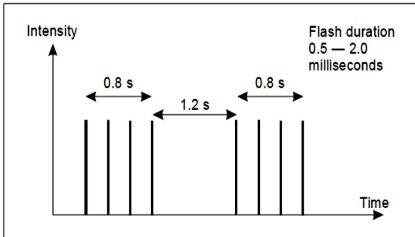
Figure 5-10. Heliport beacon flash characteristics
