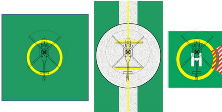
Figure 5-7. (Left) multidirectional TDPC with no limitations. (Centre) unidirectional marking shoulder line with associated centerline. (Right) multidirectional TDPC with prohibited landing sector marking
