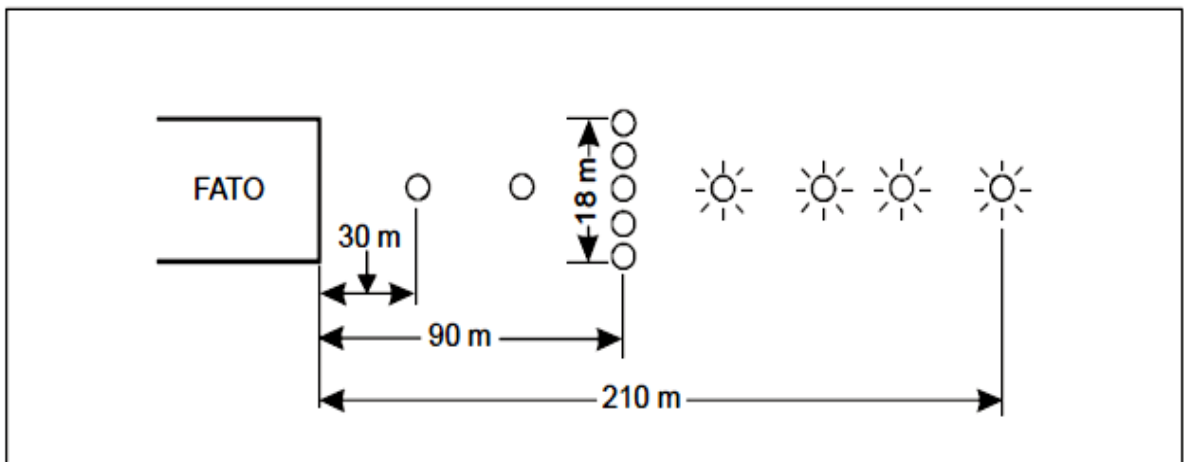
Figure 5-12. Approach lighting system
