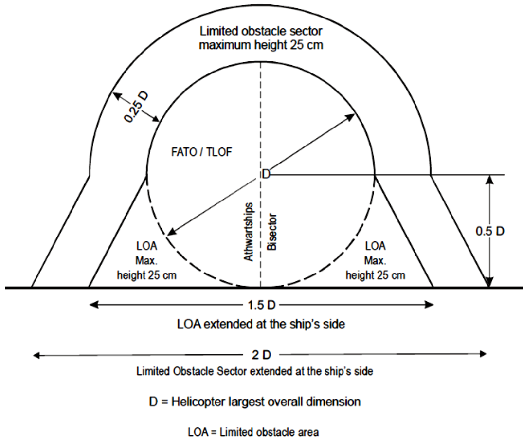
Figure 4-11. Ships-side non-purpose-built heliport obstacle limitation sectors and surfaces
