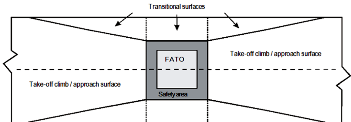
Figure 4-2. Take-off climb/Approach surface width
