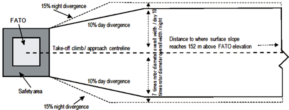
Figure 4-2. Take-off climb/Approach surface width
