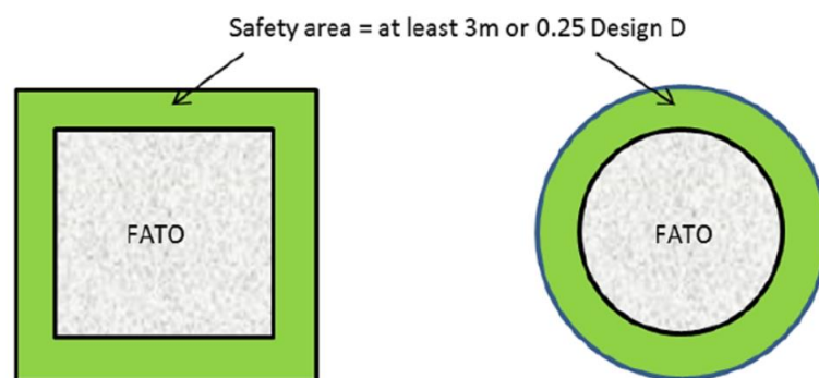
Figure 3-1. FATO and associated safety area
