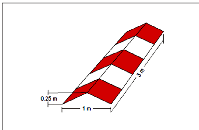
Figure 5-5. Runway-type FATO edge marker
