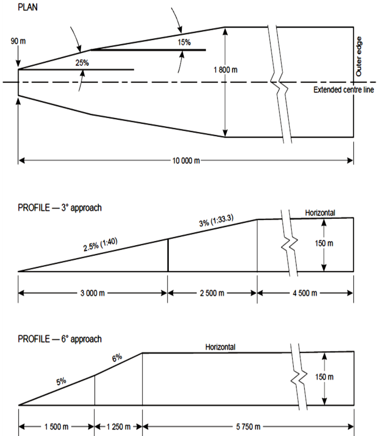
Figure A2-3. Approach surface for precision approach FATO
