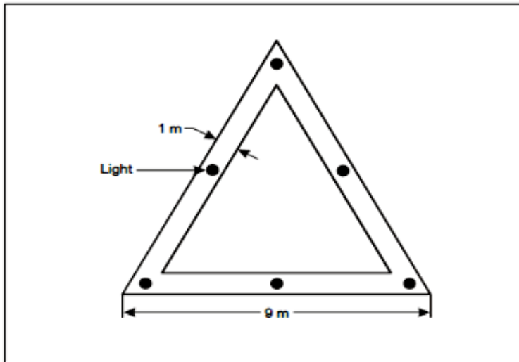
Figure 5-6. Aiming point marking
