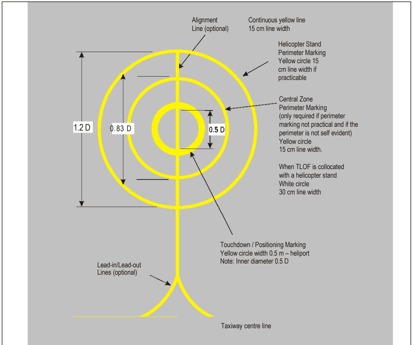
Figure 5-8. Helicopter stand markings
