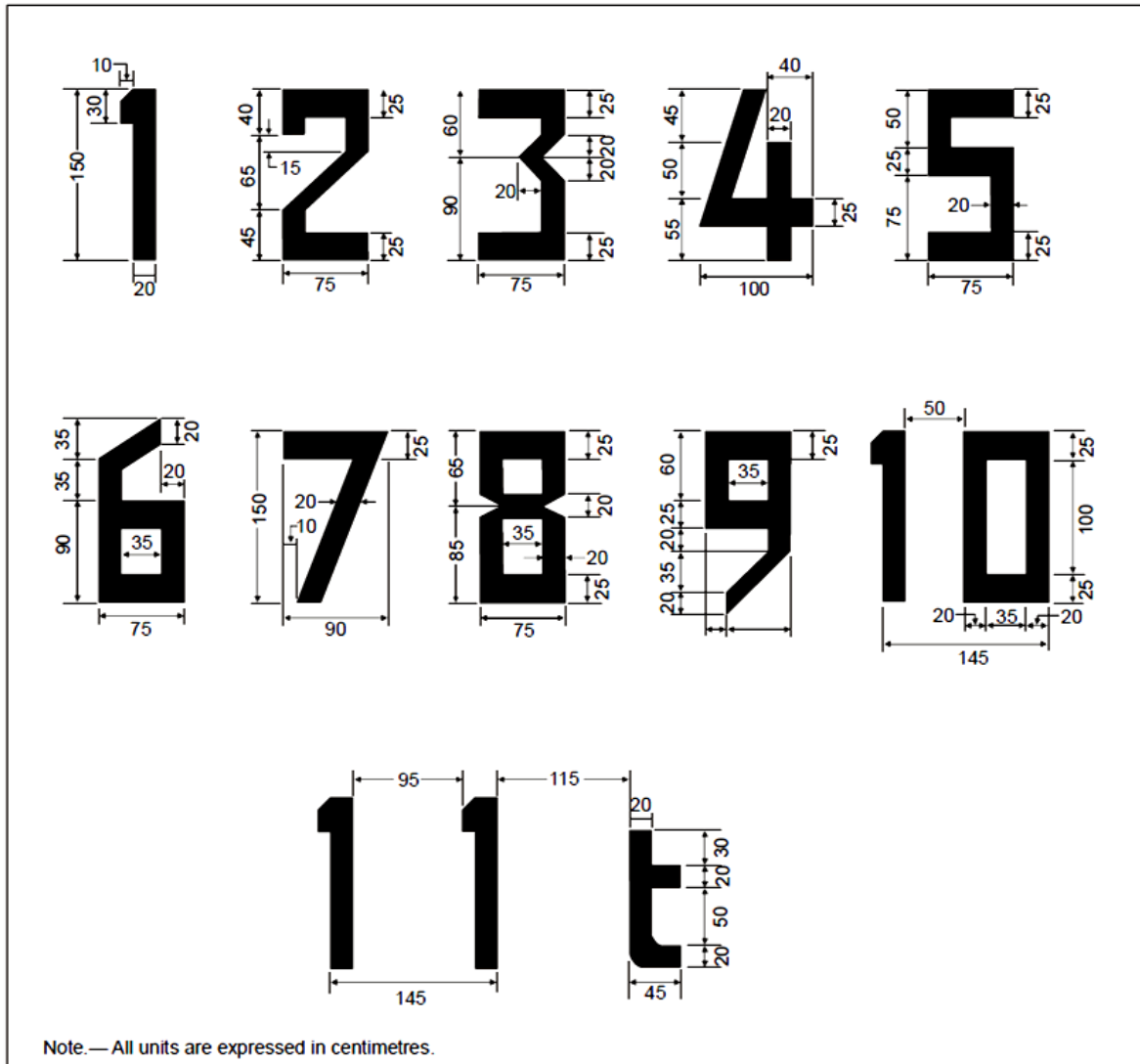
Figure 5-4. Form and proportions of numbers and letters
